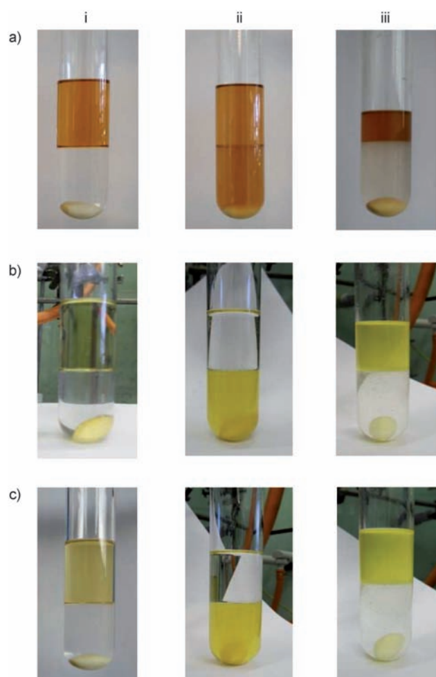
Figure 1. Phase switching after the hydroformylation of 1-octene catalyzed by rhodium complexes of a) 2 ; b) 2 and 1 combined, cycles 1a and 1b; c) 2 and 1 combined, cycle 2. i) Reaction solution with water added. ii) After bubbling CO 2 through the mixture for 1.5 h. iii) After phase separation, addition of fresh toluene, and bubbling N 2 through the mixture at 60°C for 1.5 h. The top (organic) phase from biii) was used for the hydroformylation of 1-octene to give the product phase shown in c i).
