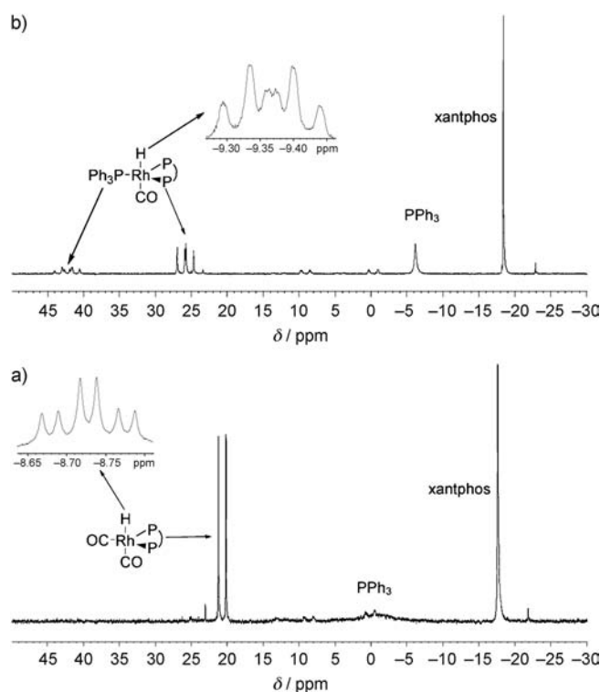
Figure 2. 31 P{ 1 H} NMR and the hydride region of the 1 H NMR spectra (inset) that were measured at room temperature for a mixture of [Rh(acac)(CO) 2 ], PPh 3 , and xantphos (1:2:2) a) Under CO/H 2 (1:1, 15 bar) and b) The solution from a) after bubbling CO 2 through the solution for 15 min.
