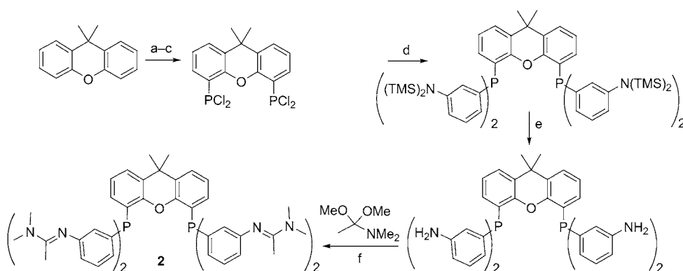
Scheme 3. Synthesis of 2 : a) THF, BuLi, −78 °C to RT, 24 h; b) (NEt 3 ) 2 PCl 2 , −78 °C to RT, 24 h; c) HCl (g) , 0 °C, 15 min; d) 3-[bis(trimethylsilyl)amino]phenylmagnesium chloride, −78 °C to RT 12 h, 55 °C, 12 h; e) MeOH, reflux, overnight; f) Microwave, 160 °C, 1 h. TMS = trimethylsilyl.
